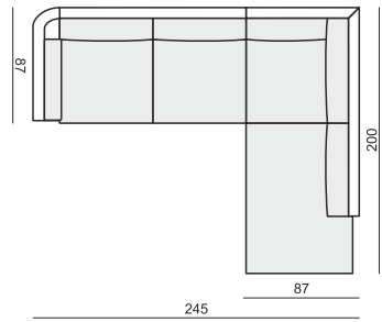
SET 3 RIGHT (or LEFT) 2 SEATER LEFT (or RIGHT) + DIVAN RIGHT (or LEFT)
